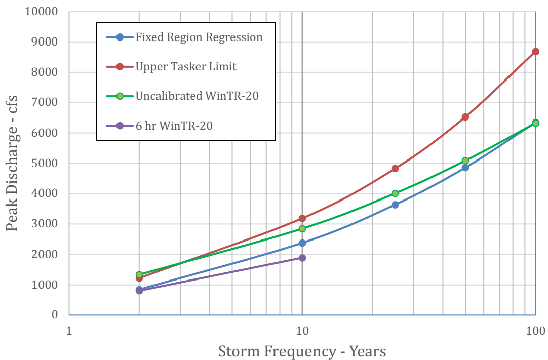
Figure A5-10 Comparison of Win TR-20 flood discharges without calibration to the Fixed Region regression estimates
