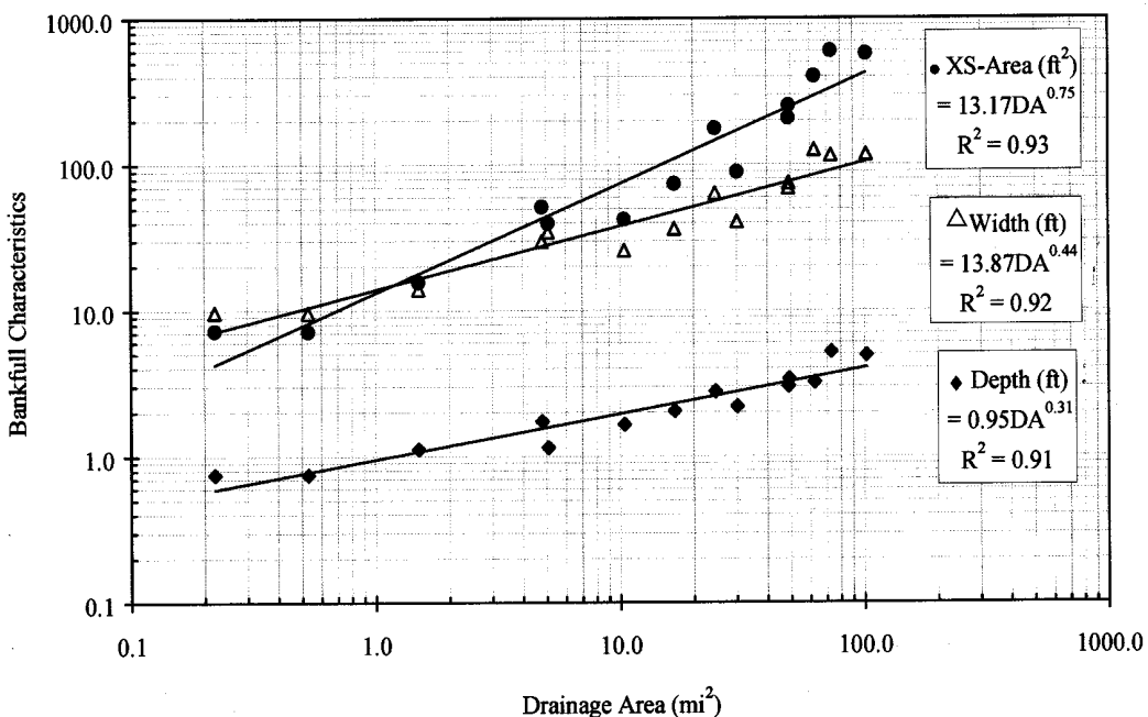
Figure A4-2: Bankfull channel dimensions as functions of drainage area for Appalachian Plateau / Valley & Ridge survey sites (n = 14) [from McCandless (2003)]
