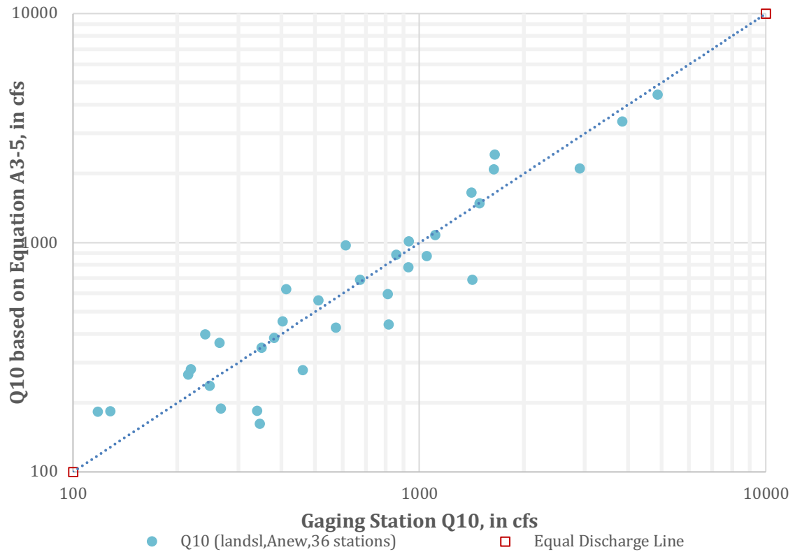
Figure A3-7: The 10-year regression estimates from Equation A3-5 plotted versus the 10-year estimates based on the gaging station data for 36 stations in the Eastern Coastal Plain Region
