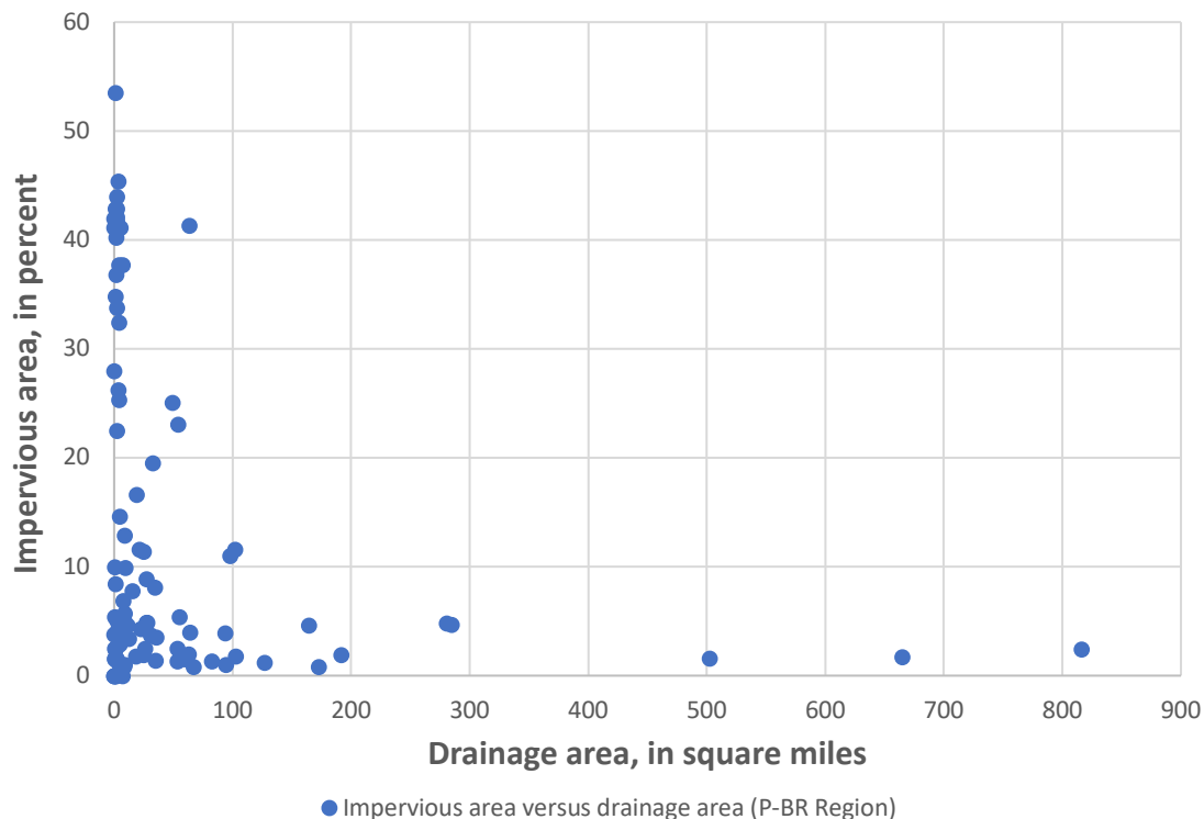
Figure 4-4: Relation of impervious area and drainage area for 96 gaged watersheds in the Piedmont-Blue Ridge Region of Maryland
