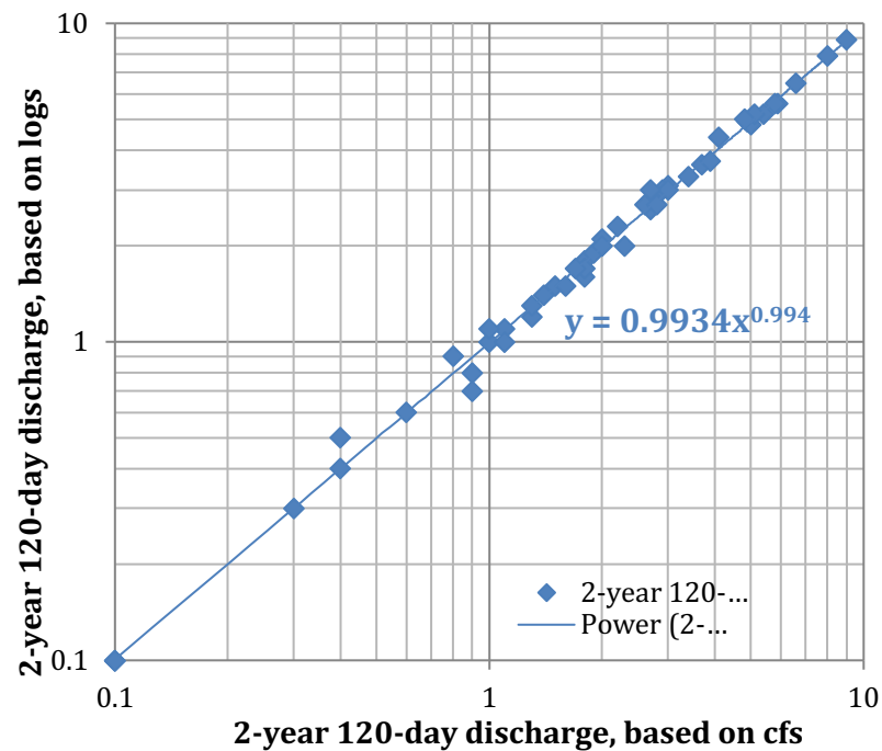
Figure 5-2: Comparison of the 2-year 120-day discharges based on the logarithmic transformed (logs) and the untransformed analysis (cfs values)
