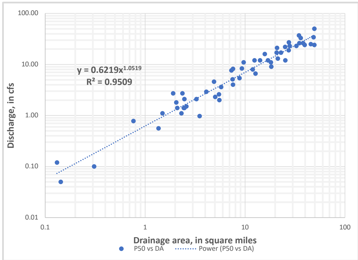
Figure 5-11: Relation between the 50-percent flow duration and drainage area for 57 gaging stations in Maryland with drainage areas less than 50 square miles
