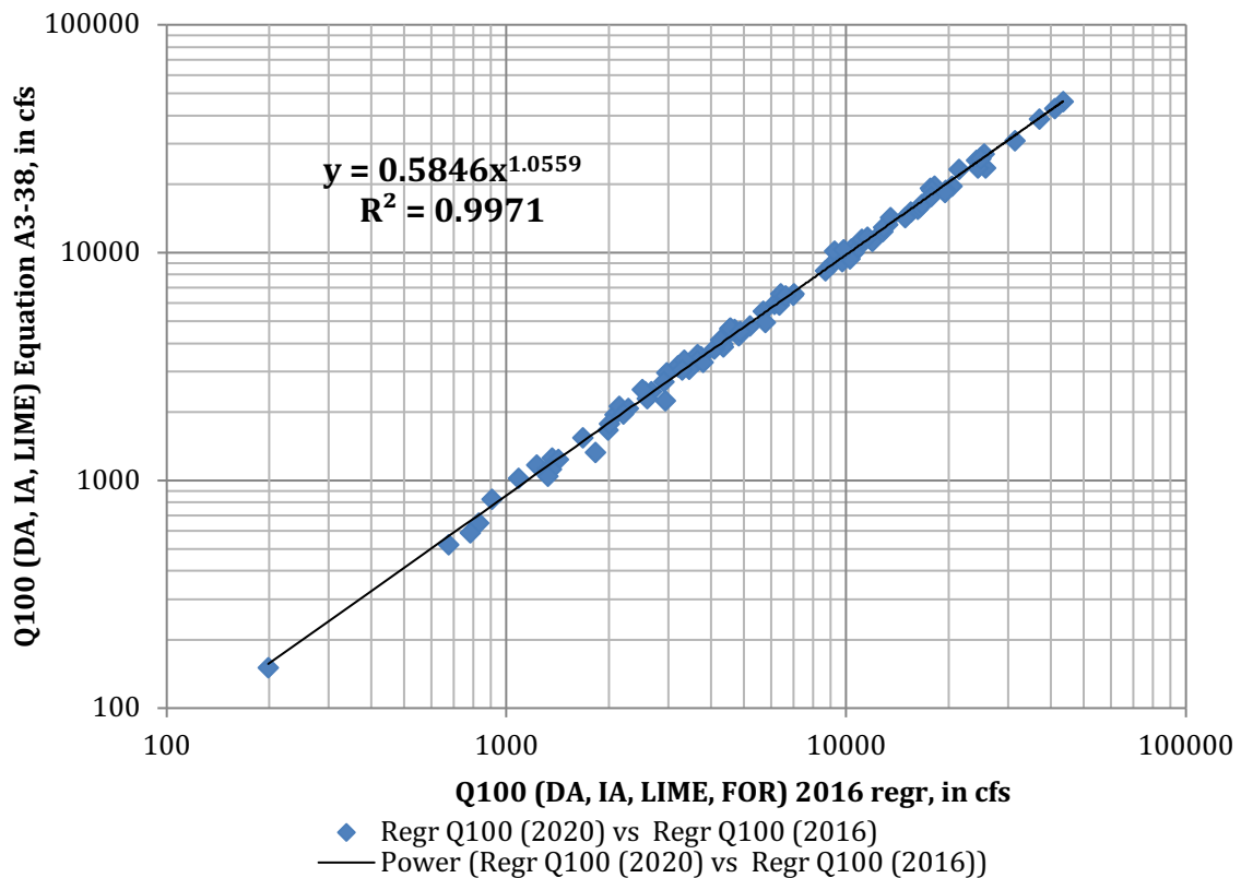
Figure A3-31: Comparison of 100-year flood discharges from Equation A3-38 to estimates from the published 2016 equation for the Piedmont-Blue Ridge Region
