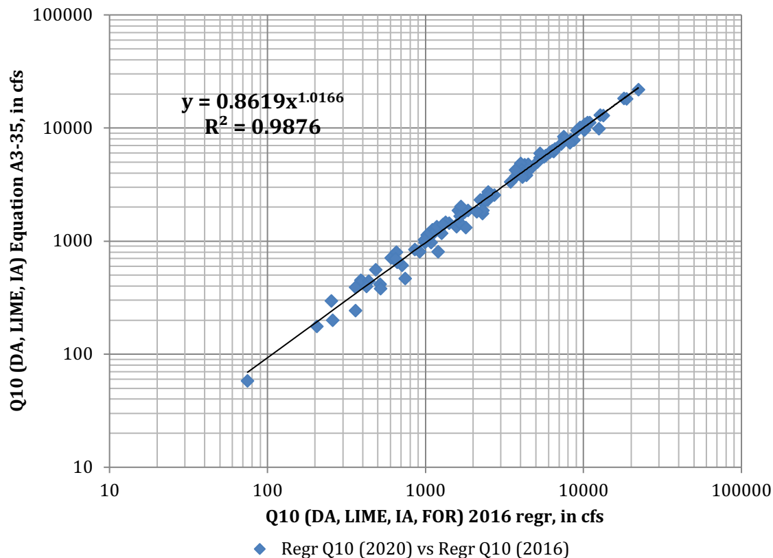
Figure A3-32: Comparison of 10-year flood discharges from Equation A3-35 to estimates from the published 2016 equation for the Piedmont-Blue Ridge Region
