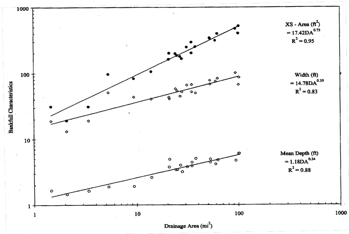
Figure A4-1: Bankfull channel dimensions as functions of drainage area for Maryland Piedmont survey sites (n = 23) (From McCandless and Everett, 2002)
