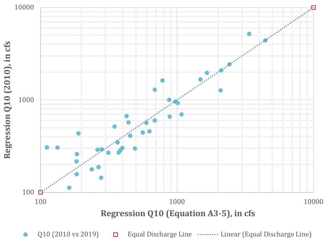
Figure A3-9: The 10-year regression estimates from the 2010 analysis versus the 10-year regression estimates based on Equation A3-5 for 41 stations in the Eastern Coastal Plain Region
