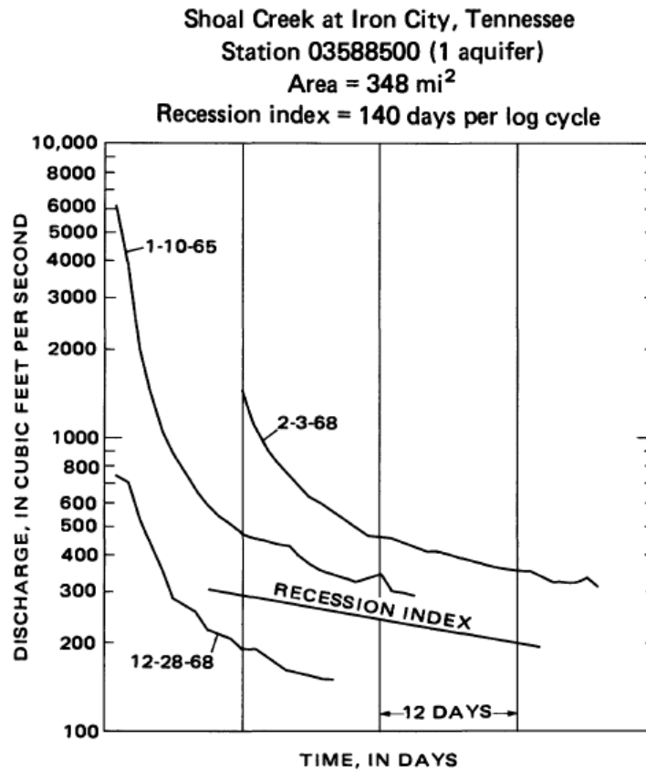
Figure 5-6: Schematic of determining the streamflow recession index
