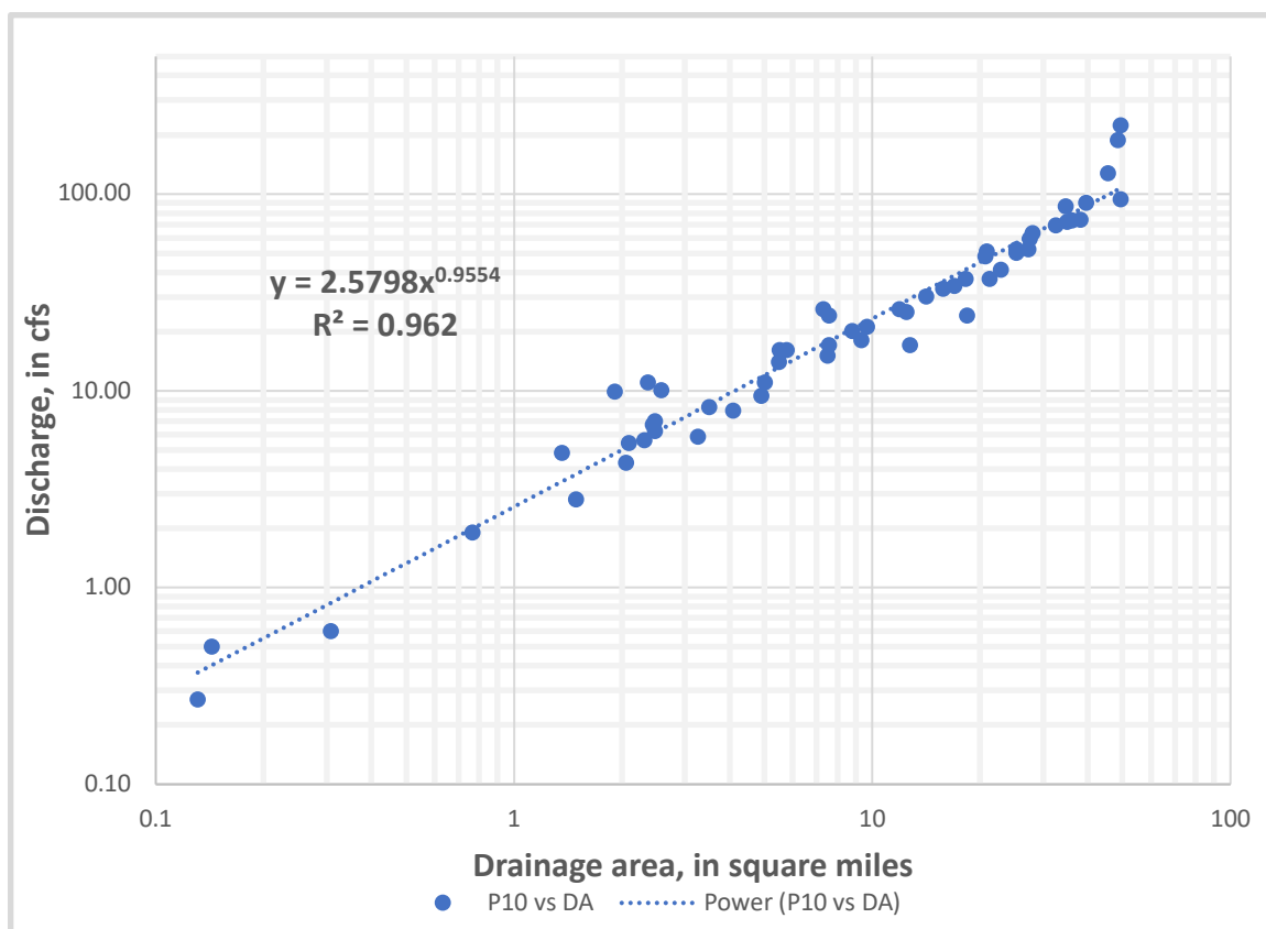
Figure 5-12: Relation between the 10-percent flow duration and drainage area for 57 gaging stations in Maryland with drainage areas less than 50 square miles
