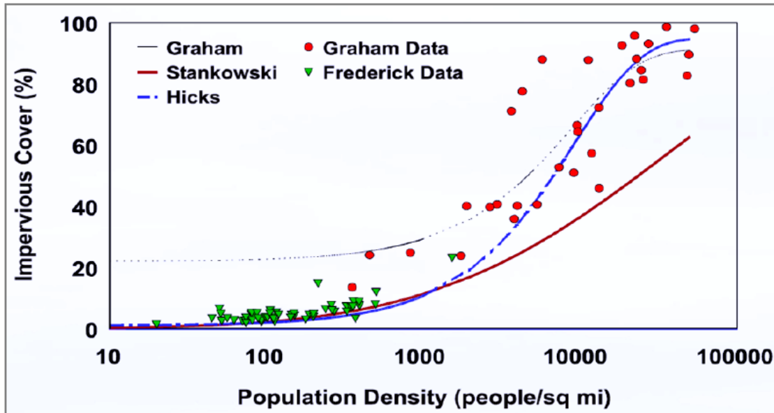
Figure 4-5: Impervious cover versus population density for several studies (from Exum and others, 2005)
