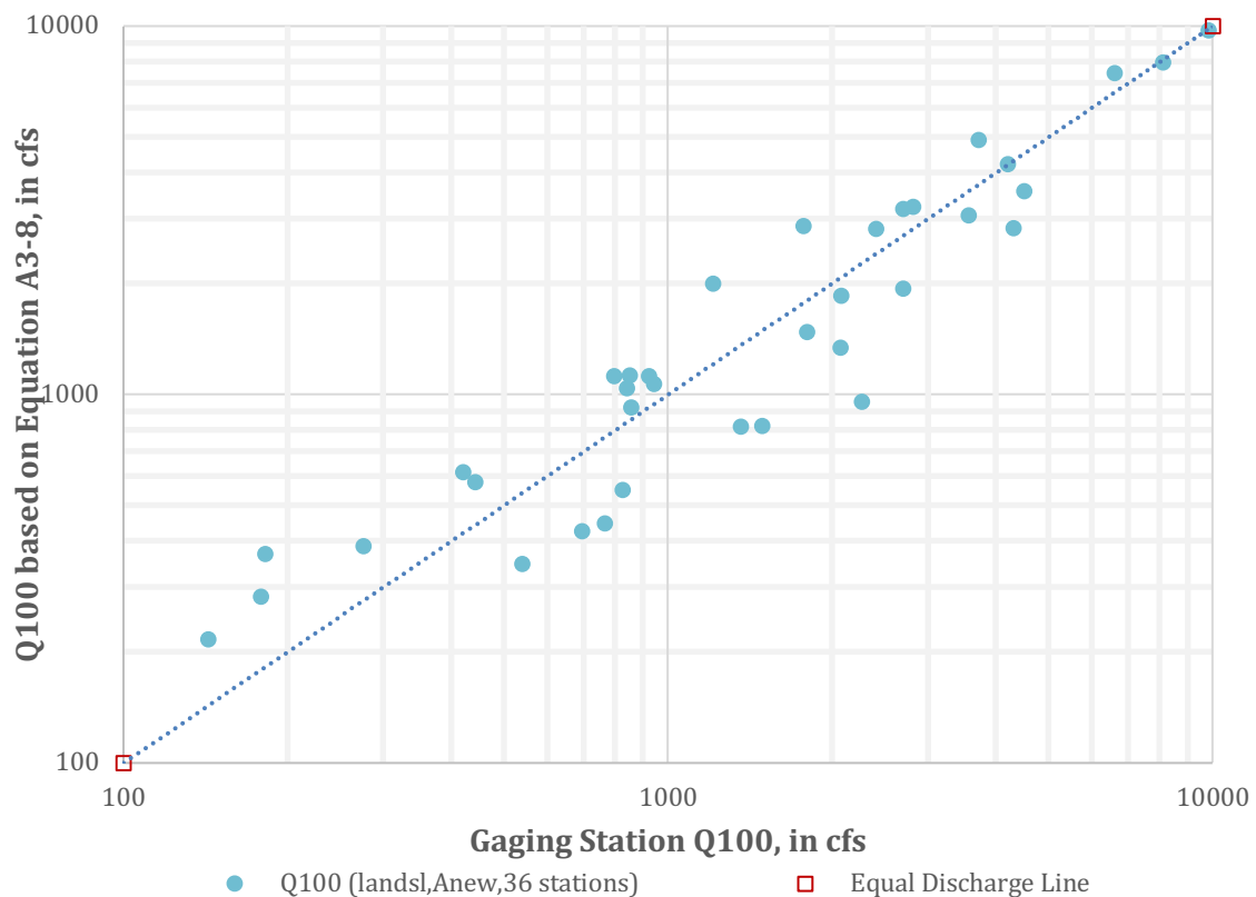
Figure A3-6: The 100-year regression estimates from Equation A3-8 plotted versus the 100-year estimates based on the gaging station data for 36 stations in the Eastern Coastal Plain Region
