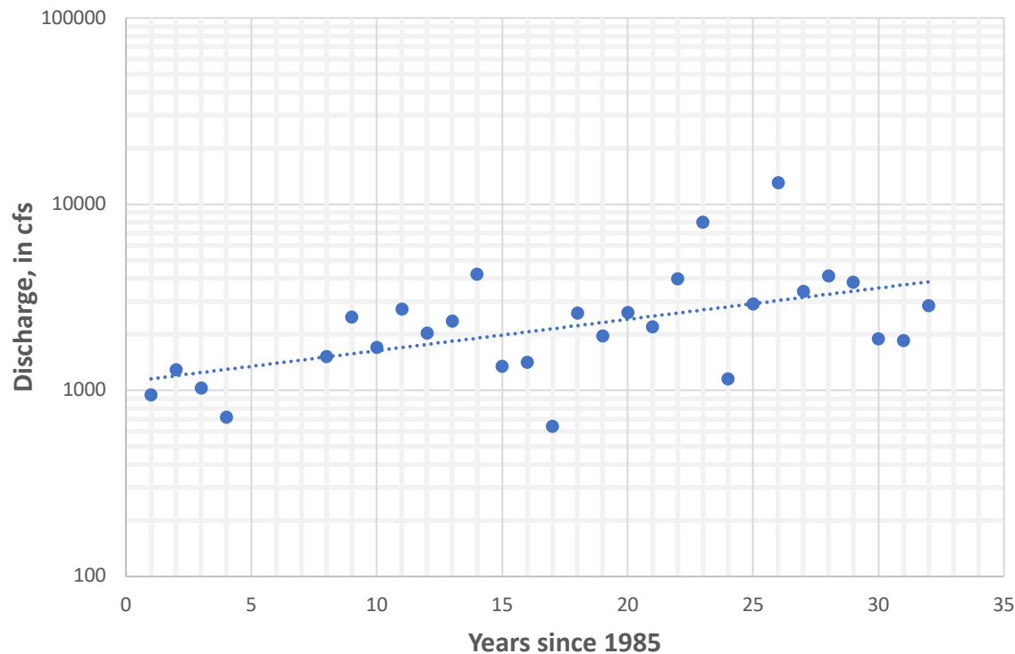
Figure A3-22: Relation between annual peak flows and years since 1985
