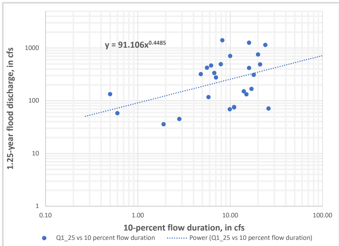
Figure 5-13: Comparison of 1.25-year flood discharge to the 10-percent flow duration percentile for 26 small watersheds in Maryland with drainage areas less than 10 square miles
