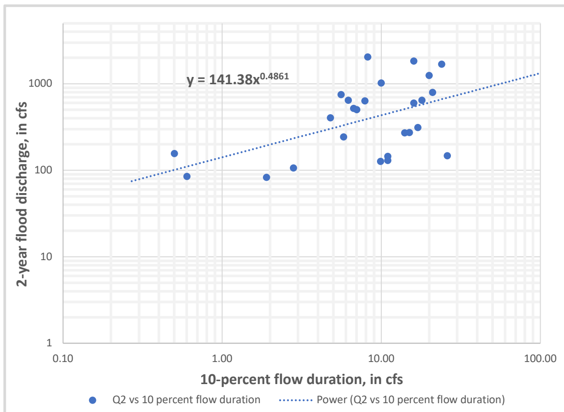
Figure 5-14: Comparison of 2-year flood discharge to the 10-percent flow duration percentile for 26 small watersheds in Maryland with drainage areas less than 10 square miles
