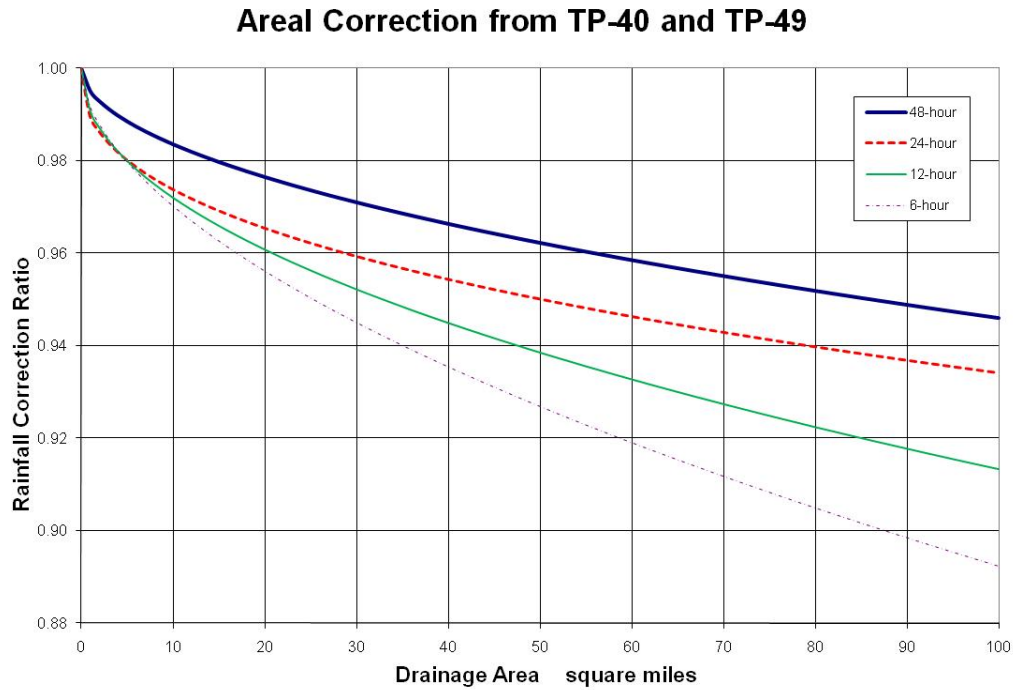
Figure 3-10: Areal Reduction curves based on TP-40
