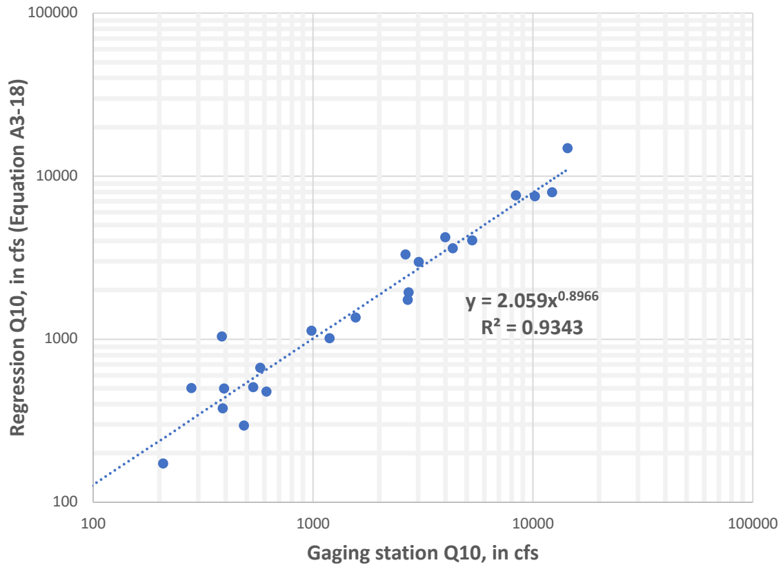
Figure A3-19: The 10-year regression estimates from Equation A3-18 plotted versus the 10-year estimates based on gaging station data for 23 stations in the Western Coastal Plain Region
