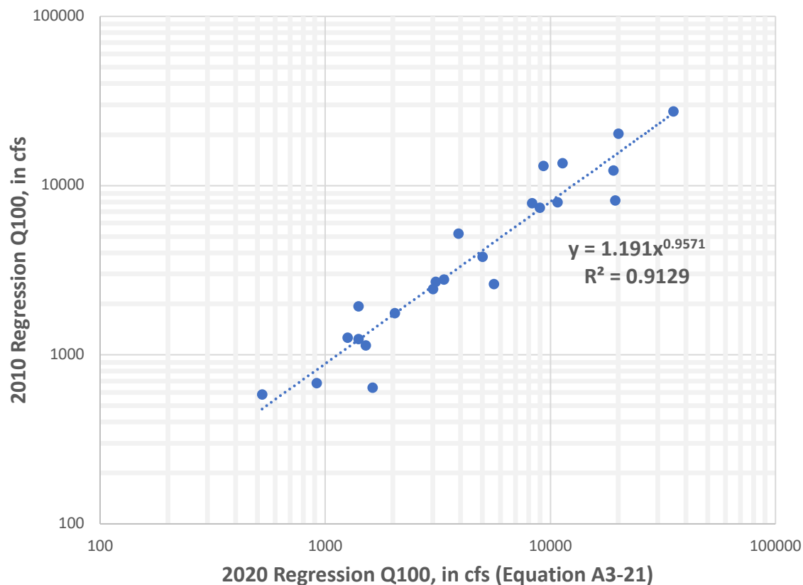
Figure A3-20: Comparison of the 100-year flood discharges for the 2010 and 2020 regression equations
