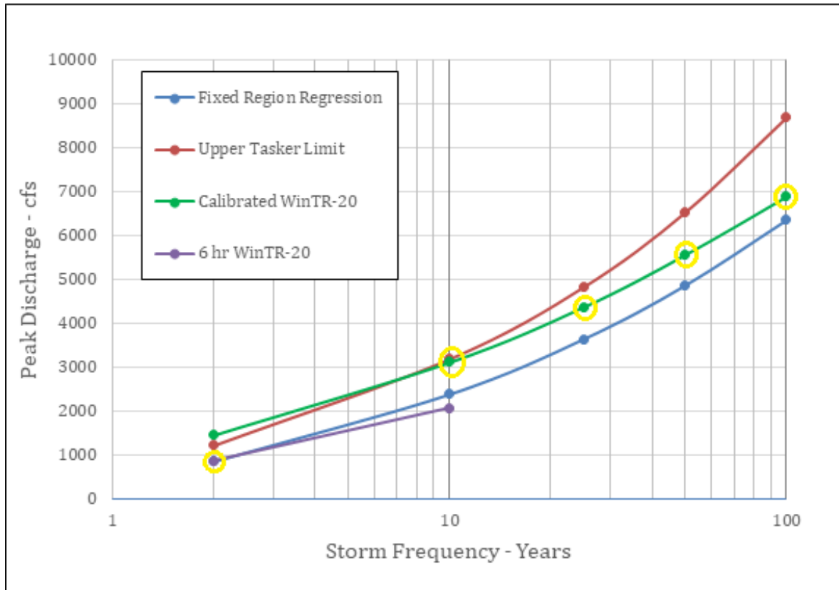
Figure A5-11 Final calibrated Win TR-20 flood discharges as compared to the Fixed Region regression estimates
