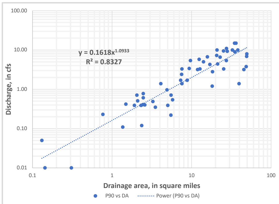
Figure 5-10: Relation between the 90-percent flow duration and drainage area for 57 gaging stations in Maryland with drainage areas less than 50 square miles
