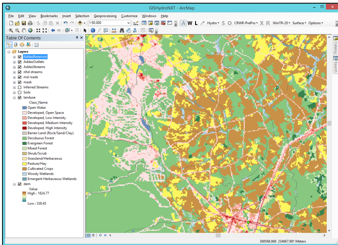
Figure A5-3 Distribution of land use data from the NLCD 2001 database
