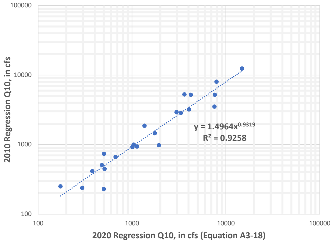
Figure A3-21: Comparison of the 10-year flood discharges for the 2010 and 2020 regression equations
