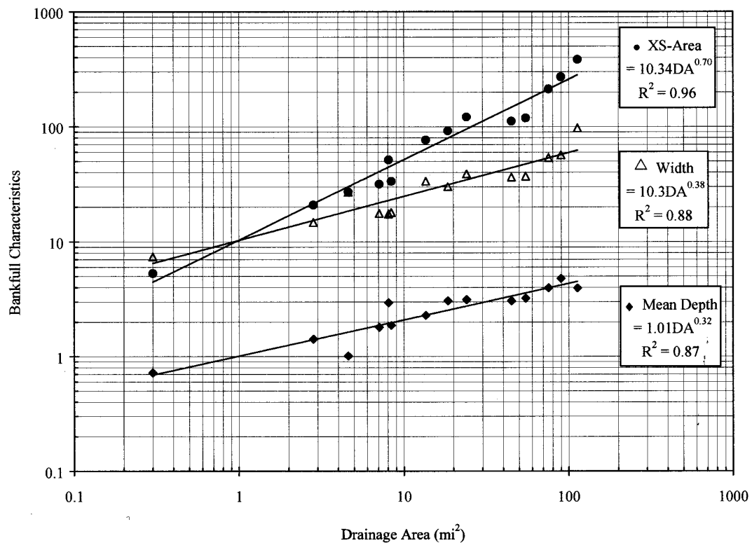
Figure A4-3: Bankfull channel dimensions as functions of drainage area for Coastal Plain survey sites (n = 14) [from McCandless (2003)]
