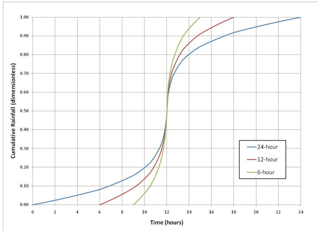
Figure 3-9: 6-, 12-, and 24-Hour Storm Distributions Howard County MD
