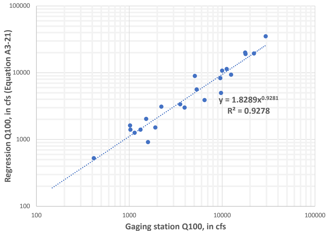
Figure A3-18: The 100-year regression estimates from Equation A3-21 plotted versus the 100-year estimates based on gaging station data for 23 stations in the Western Coastal Plain Region
