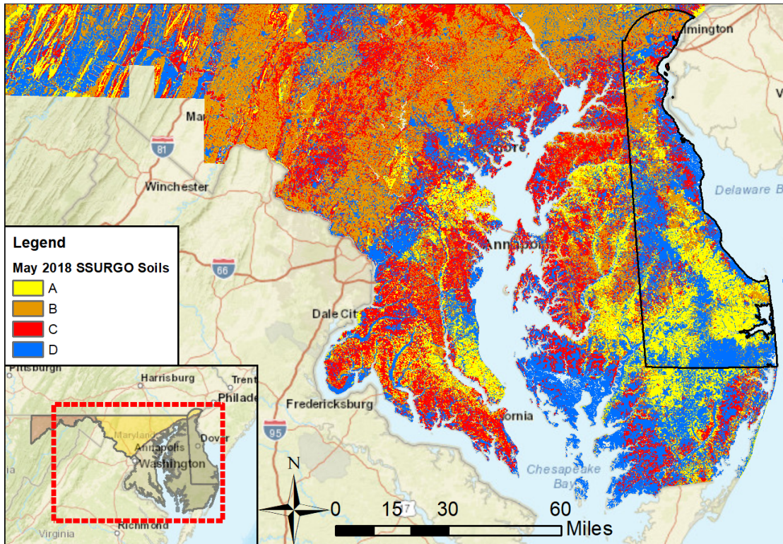
Figure A3-16: The May 2018 SSURGO soils data
