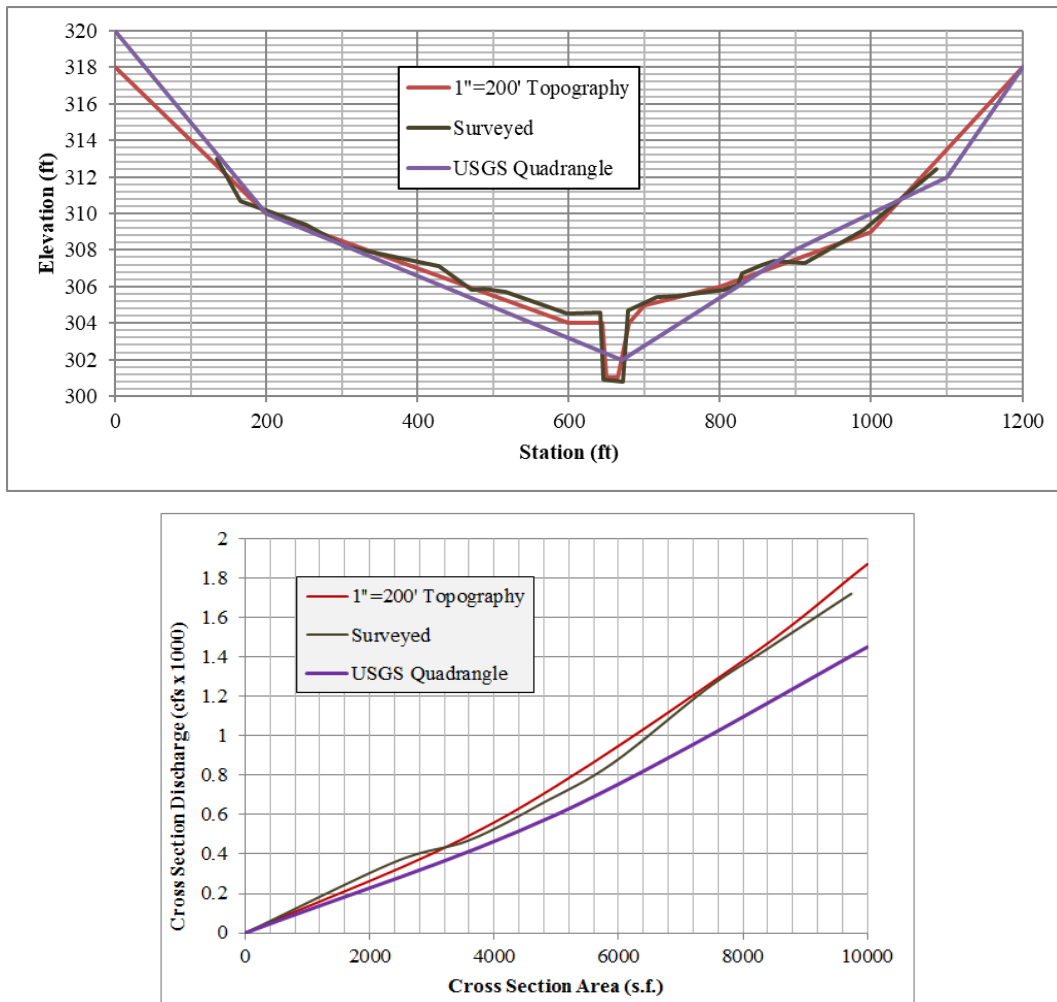
Figure 3-8: Discharge-Area Curves for Surveyed and Contour Defined Synthetic Cross Sections
