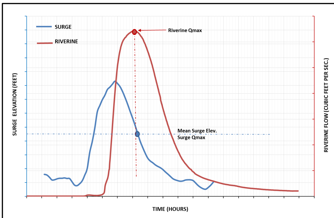
Figure 6-5: Illustration of the riverine peak discharge (Riverine Qmax) occurring at the same time as the maximum storm surge discharge (Surge Qmax)
