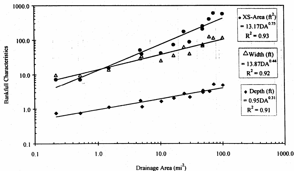
Figure 3.8 Bankfull Characteristics for Selected USGS Sites in the Maryland Piedmont
