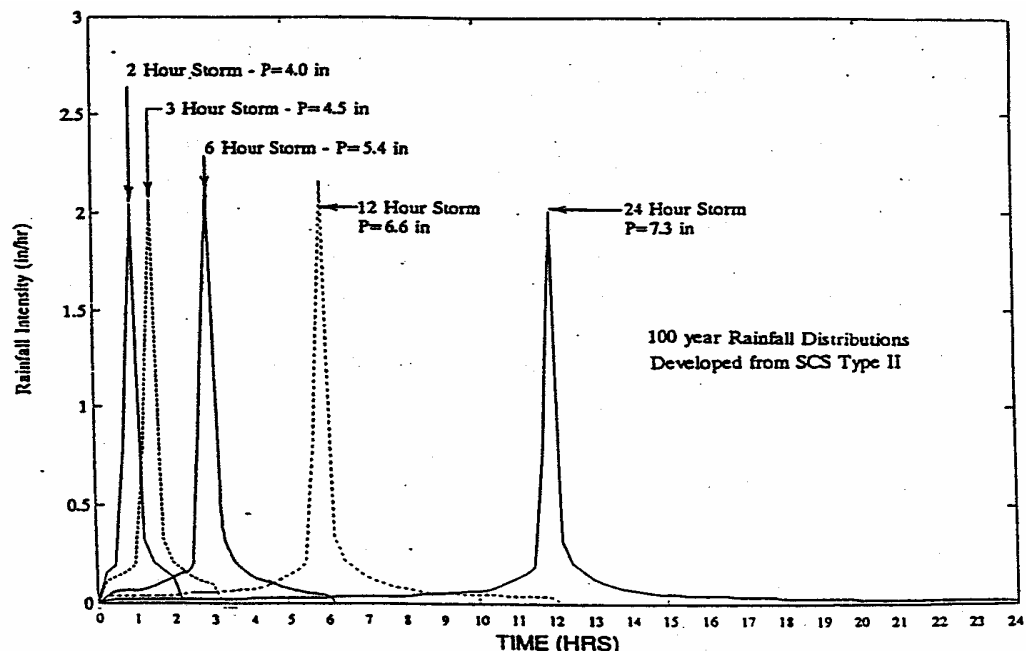
Figure 3.20 Intensities for Design Storms of Indicated Durations
