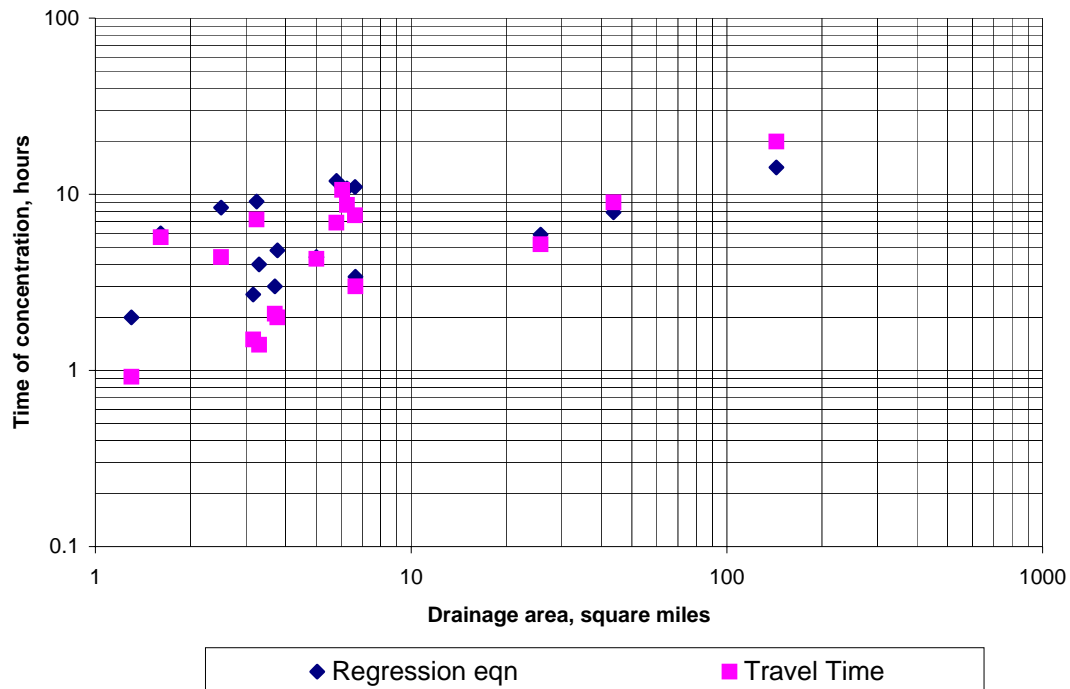
Figure A6.2. Comparison of time of concentration based on Equation 1 and the travel time method.
