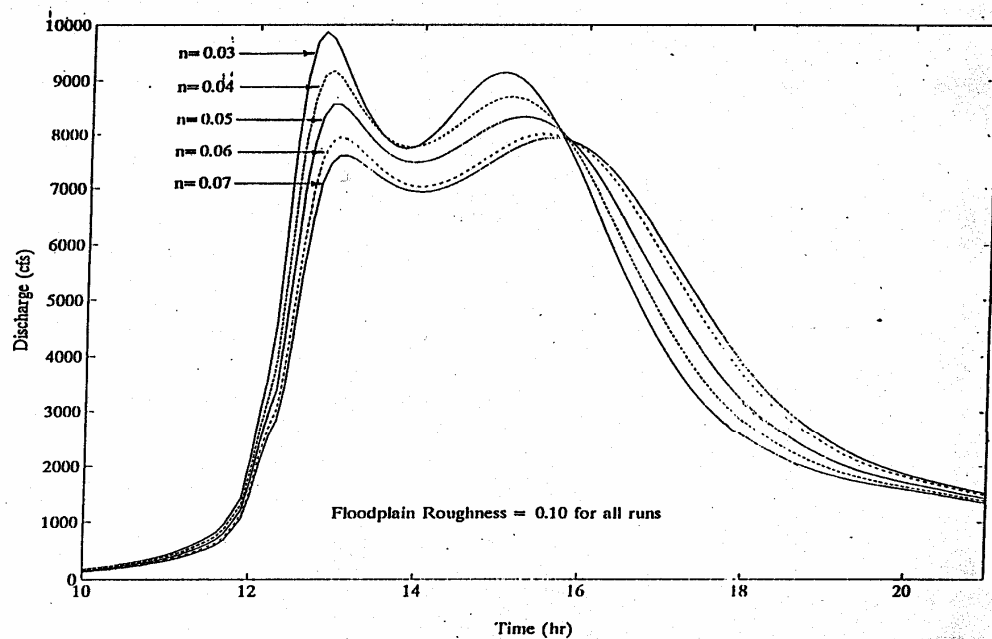
Figure 3.7 Hydrographs for a Range of In-Bank Channel Roughness Coefficients
