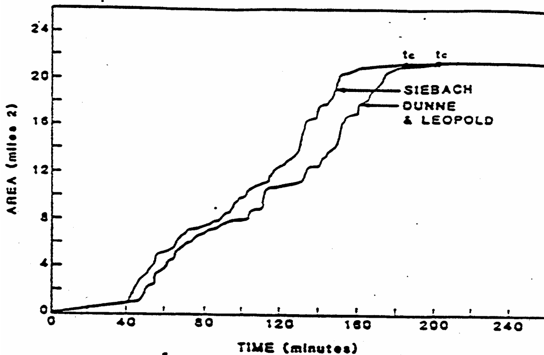
Figure 3.9 Time-Area Curves Using Surveyed and Regression Equation Defined In-Bank Cross Sections ( n=0.04 )
