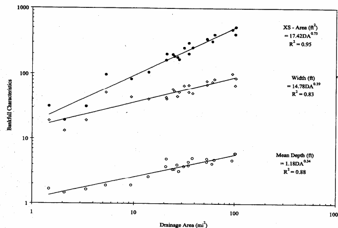
Figure 17. Bankfull channel dimensions as a function of drainage area for Maryland Piedmont survey sites (n = 23).
