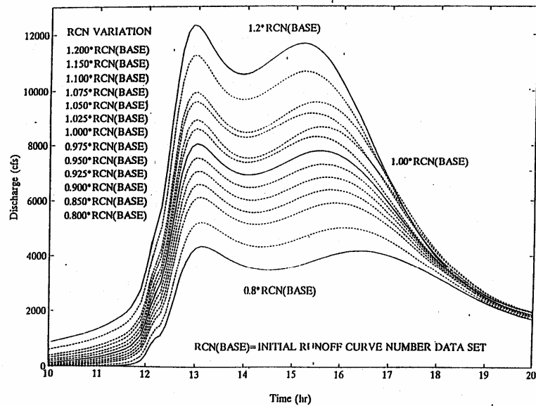
Figure 3.3 Hydrograph Response to Changing RCN
