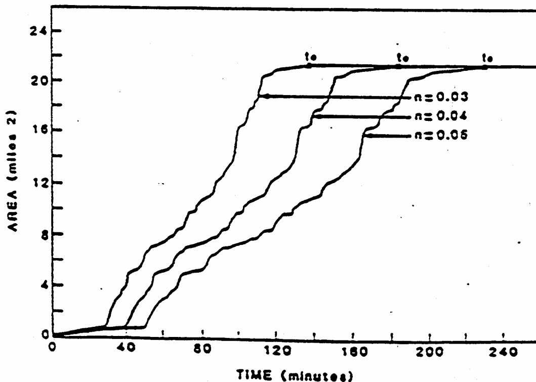
Figure 3.10 Time-Area Curves Using Surveyed In-Bank Cross Sections and Indicated Manning Roughness Coefficients
