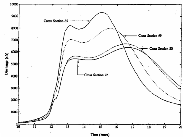
Figure 3.13 Hydrographs Generated Using a Single Cross Section to Represent the Stream
