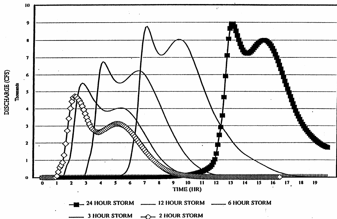
Figure 3.21 Hydrographs Using 100-yr Design Storms of Indicated Durations
