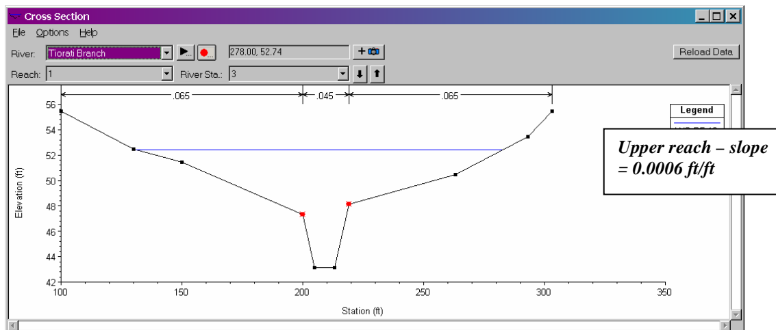
Cross Section 28 (HEC-RAS)
