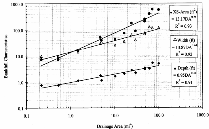
Figure 13. Bankfull channel dimensions as a function of drainage area for AP/VR survey sites ( n = 14 ).
