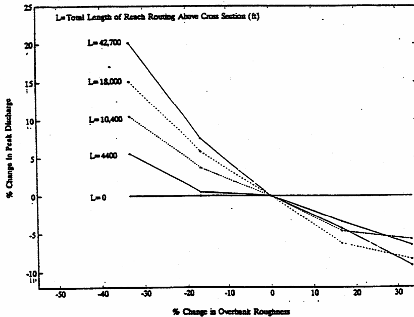
Figure 3.17 Percent Change in Peak Discharge as a Function of Channel Length and the Percent Change in the Manning Roughness Coefficient
