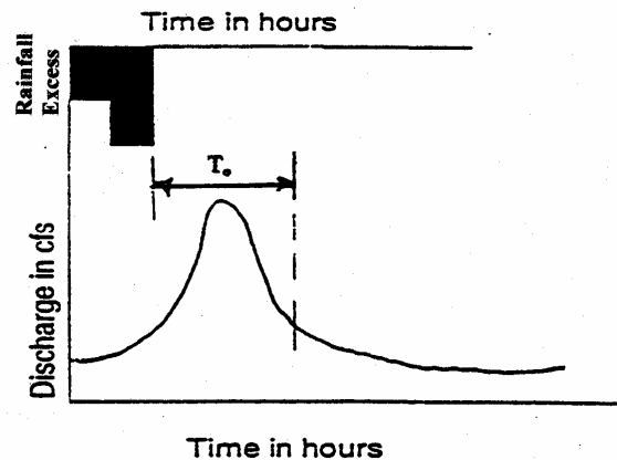
Figure 3.5 Time of Concentration
