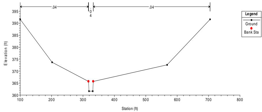
Figure A5a-2 Cross Sections Considered for Development of Stage-Discharge-Area Relations Along Routing Reach Through Sub-Watershed 3.
