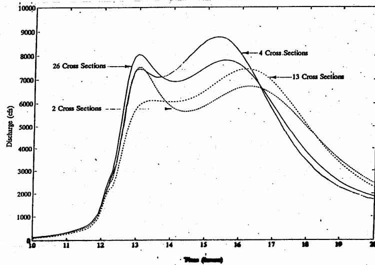
Figure 3.11 Hydrographs with Stream Network Attenuation Defined with Indicated Number of Subwatersheds & Routing Reaches
