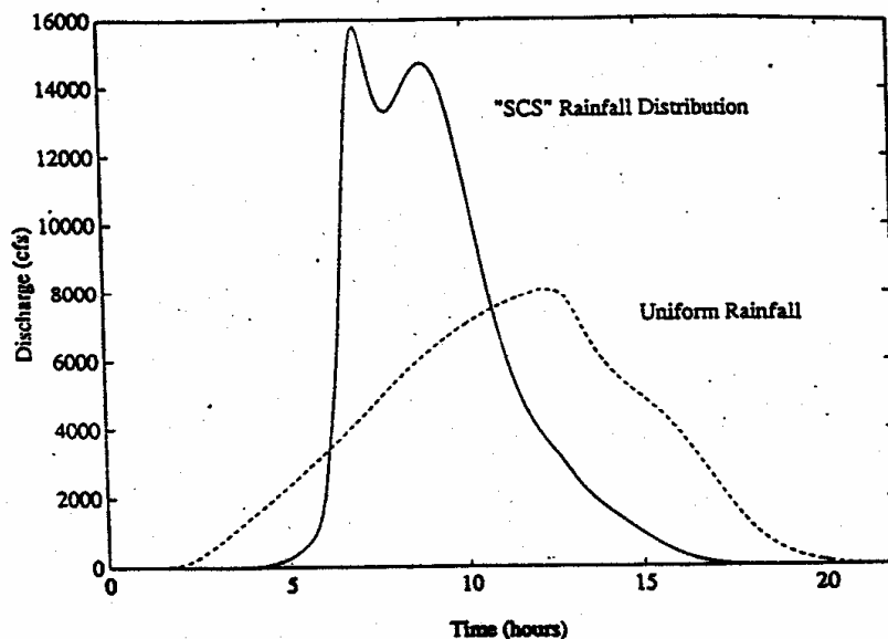
Figure 3.18 Hydrographs Produced by TR-20 Using 12-Hour Storms of 8.5 Inches as Input
