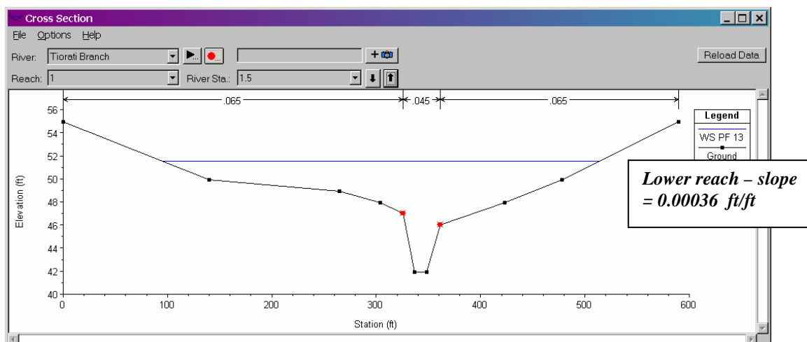
Cross Section 29 (HEC-RAS)
