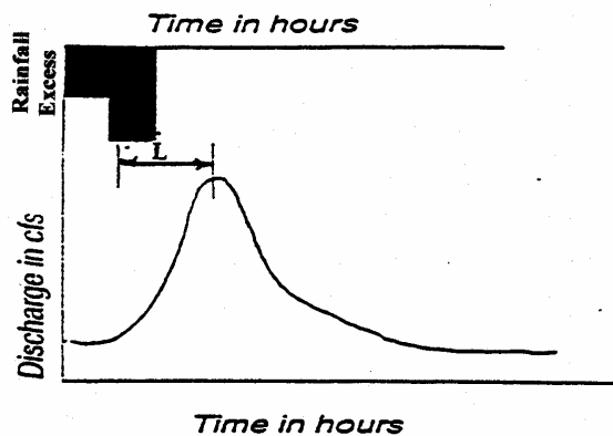
Figure 3.4 Definition of Lag Time
