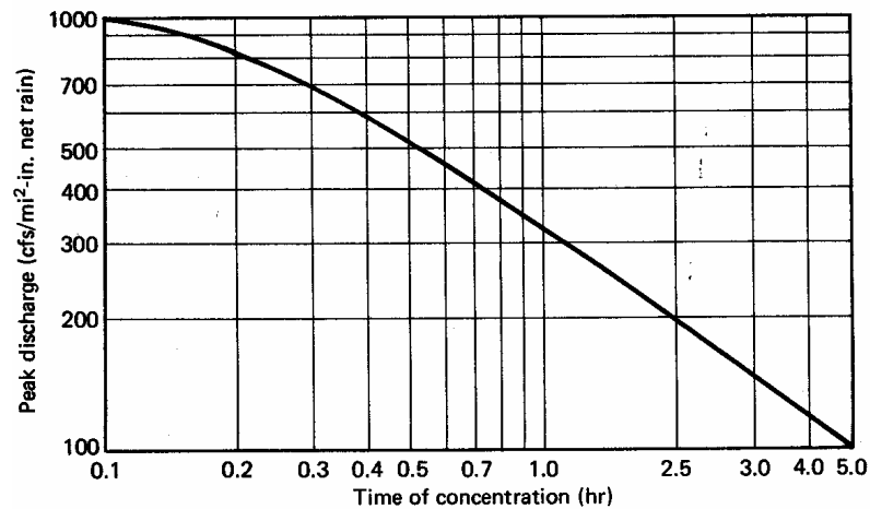
Figure 3.6 Peak Discharge in CSM per Inch of Runoff Vs. Time of Concentration for a 24-Hour Type II Storm Distribution (From Viessman, Lewis and Knapp((1989))
