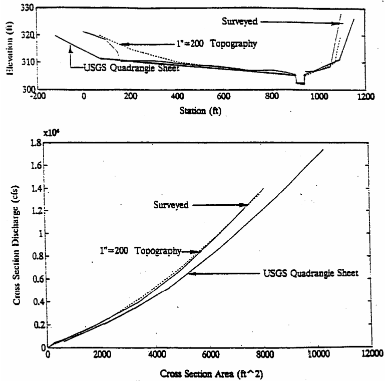
Figure 3.14 Discharge-Area Curves for Surveyed and Contour Defined Synthetic Cross Sections
